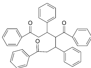
Kostanecki's triketone
